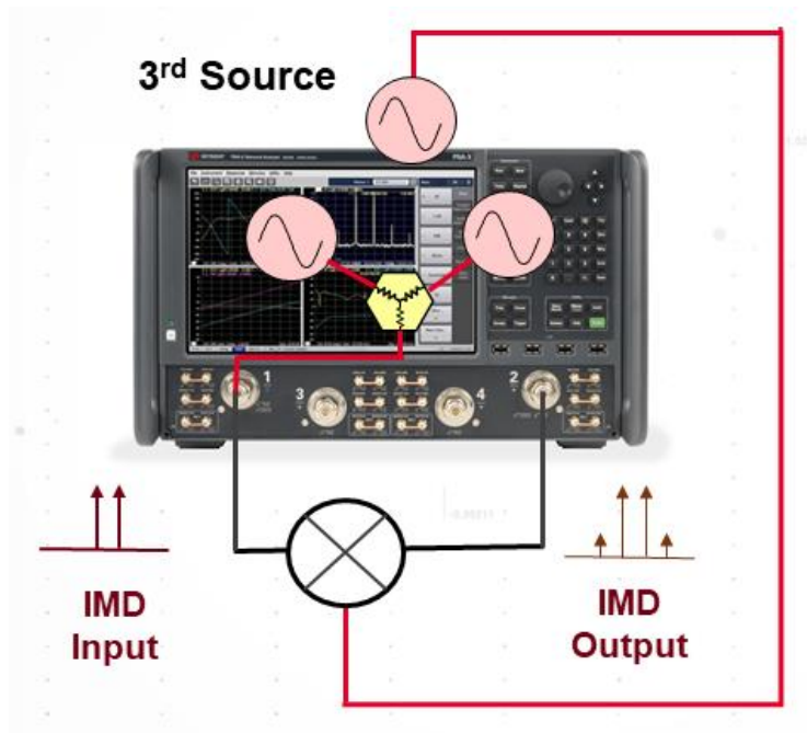
Figure 4. Two-tone IMD mixer measurement
