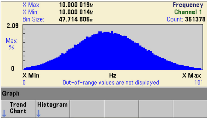
FIGURE 2: Histogram graph on a 53230A
