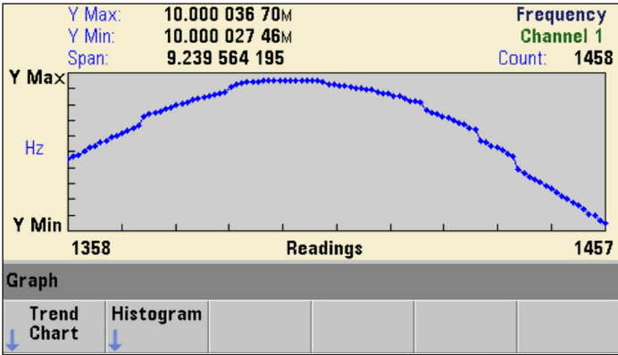
FIGURE 1: Trend chart on a 53230A
