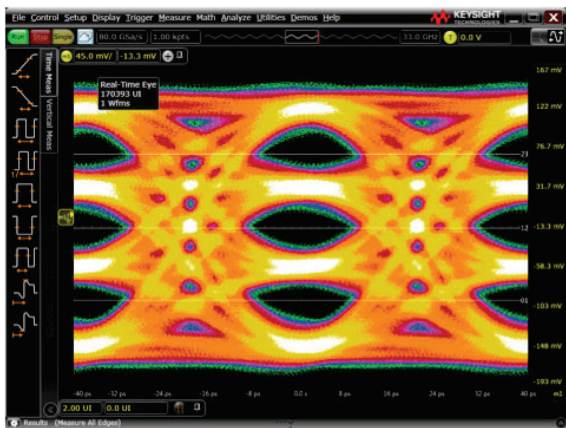
Figure 2: the bit-slice of this, showing the transition states overlapped, which creates an eye diagram
