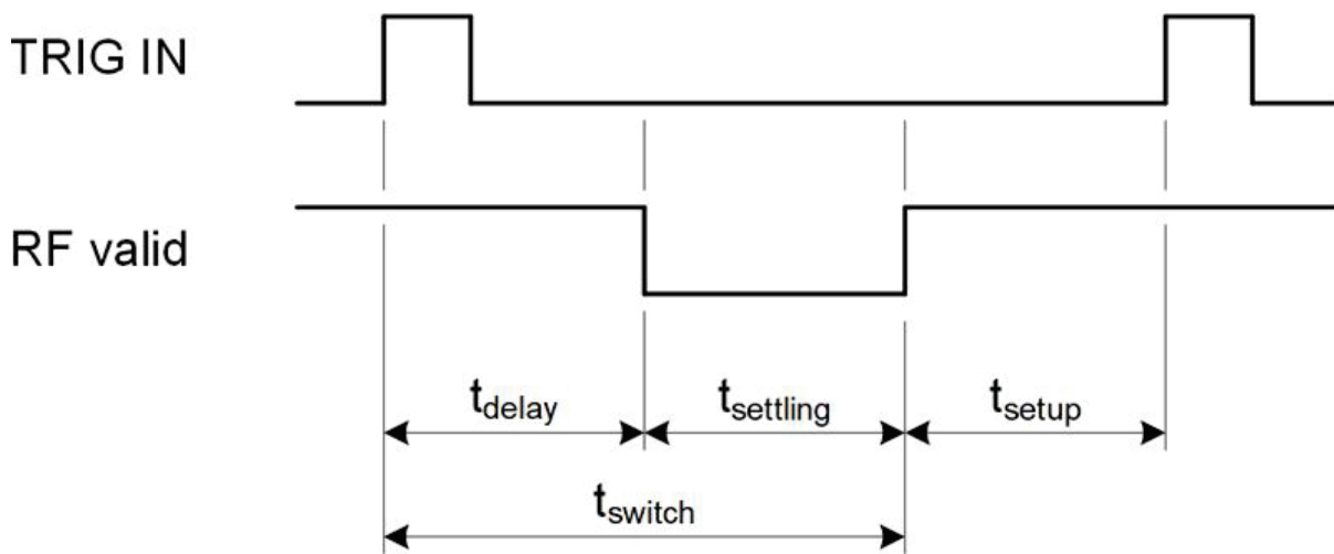
Figure 14. Timing diagram
