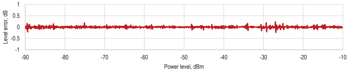
Figure 10. Relative power level accuracy at 20 GHz (Options 520 and 1E1)
