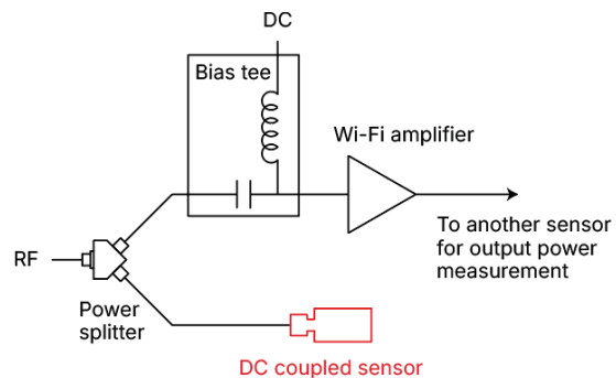
Figure 1(b). A bias tee has to be connected after the power splitter so that the DC component is blocked from entering the DC-coupled sensor.
