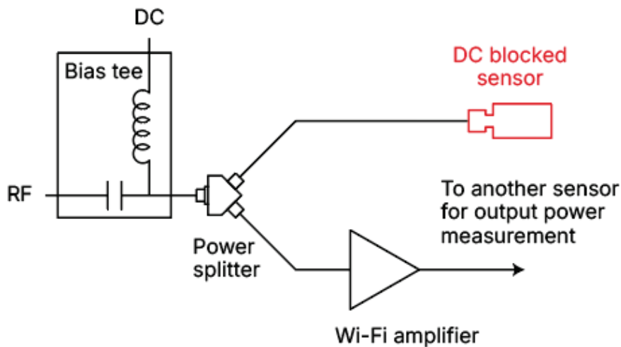
Figure 2. A DC-blocked sensor is a more appropriate equipment to measure the input power of the amplifier.
