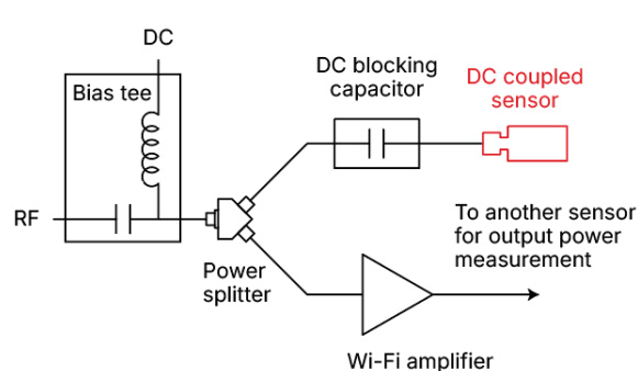
Figure 1(a). An external DC blocking capacitor is required to prevent the DC component from entering the DC-coupled sensor.
