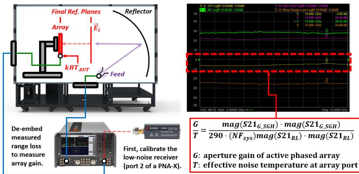
Figure 10. Diagram showing how to make noise figure measurements for receiver arrays using the PNA-X vector network analyzer.
