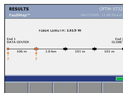
Figure 2. Advanced troubleshooting capability, such as highlighting questionable connectors in the link-under-test.
