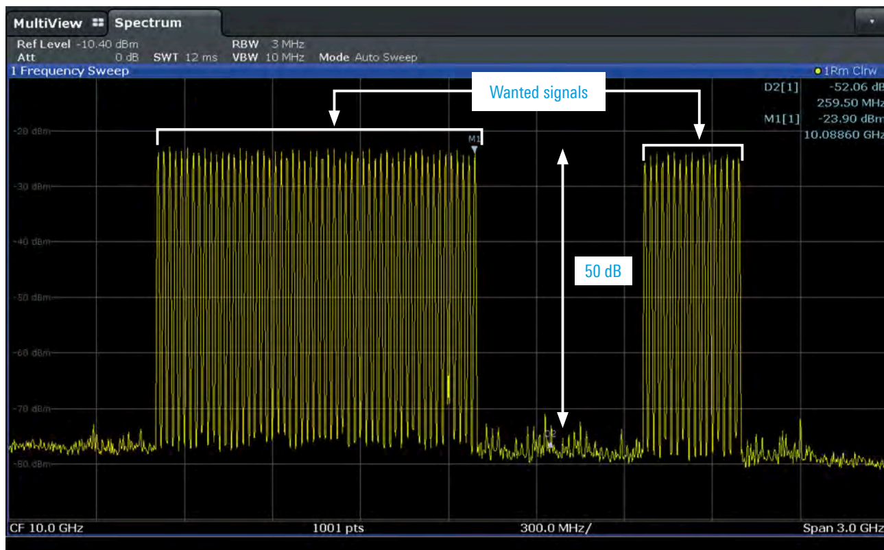
2 GHz wide multicarrier continuous wave (MCCW) signal generated with the R&S®SMW200A vector signal generator.
