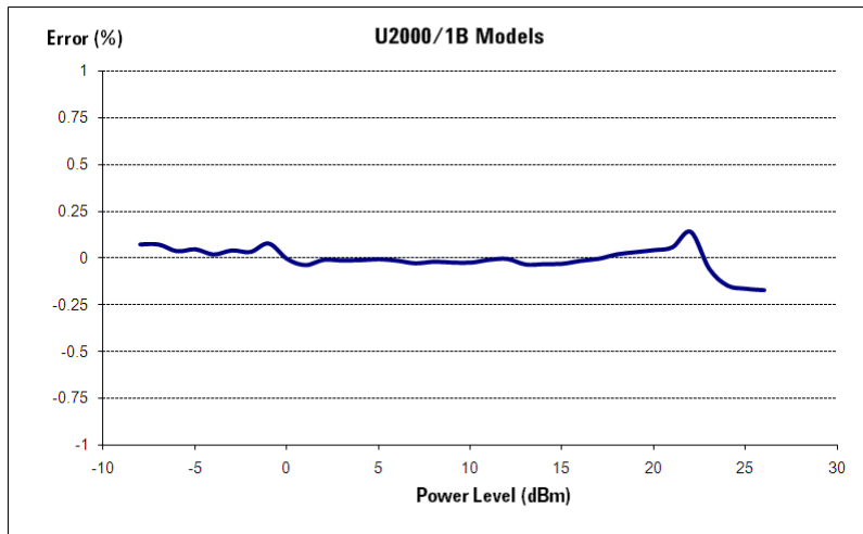
Figure 3-11 Typical power accuracy at 25 °C for U2000/1B models 1
