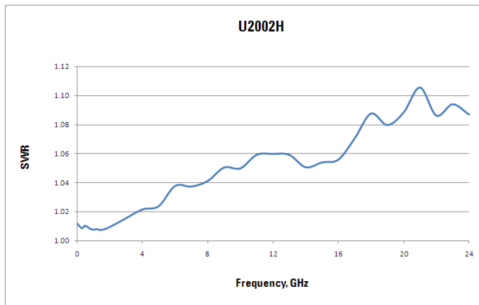
Figure 3-7 U2002H Typical SWR (25 °C ±10 °C)
